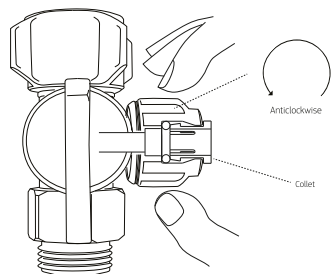
Figure 7 - SmartTee™ Quick Connect Fitting
